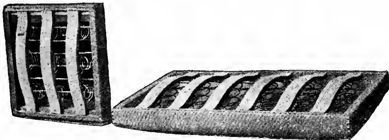
Figs. 3936-3937. REVERSE SIDE OF SINGLE AND DOUBLE RATTAN SPRING SEATS. Showing Construction.
